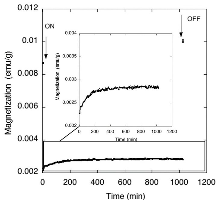
Figure 3. Time dependence of the magnetization of HNanoCoFe under irradiation ( \lambda = 635 nm).
